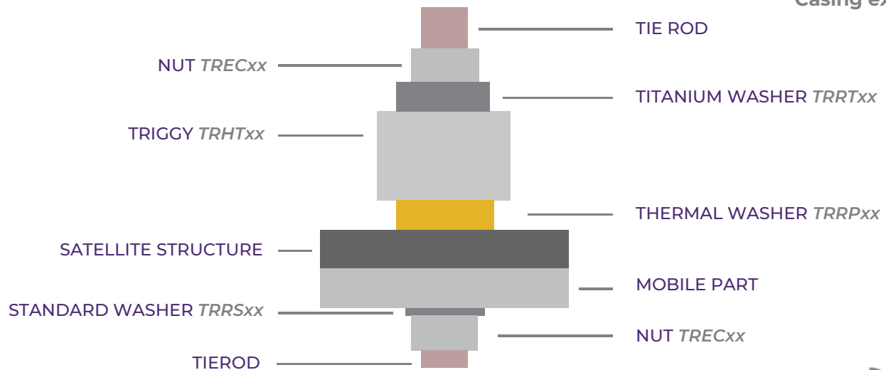
Casing example
